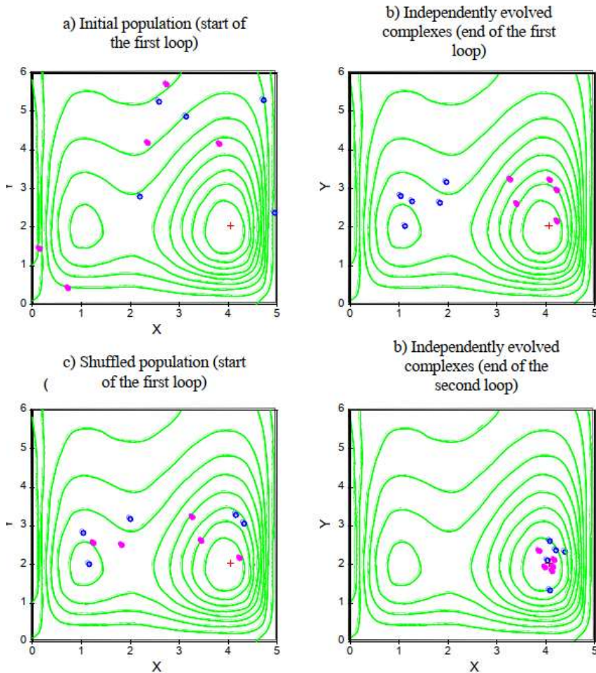
Figure B.2: Shuffled Complex Evolution (SCE) algorithm
