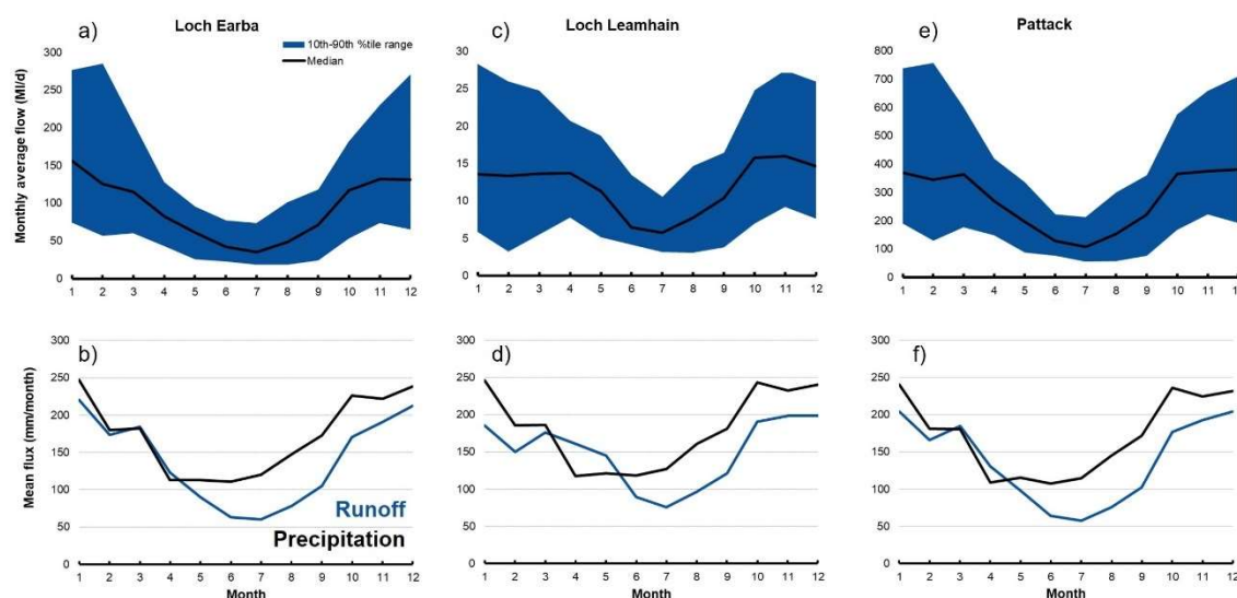
Figure 5.6: Seasonal distribution of a,c,e) total monthly flows and b,d,f) runoff and precipitation for the period 1960-2021
