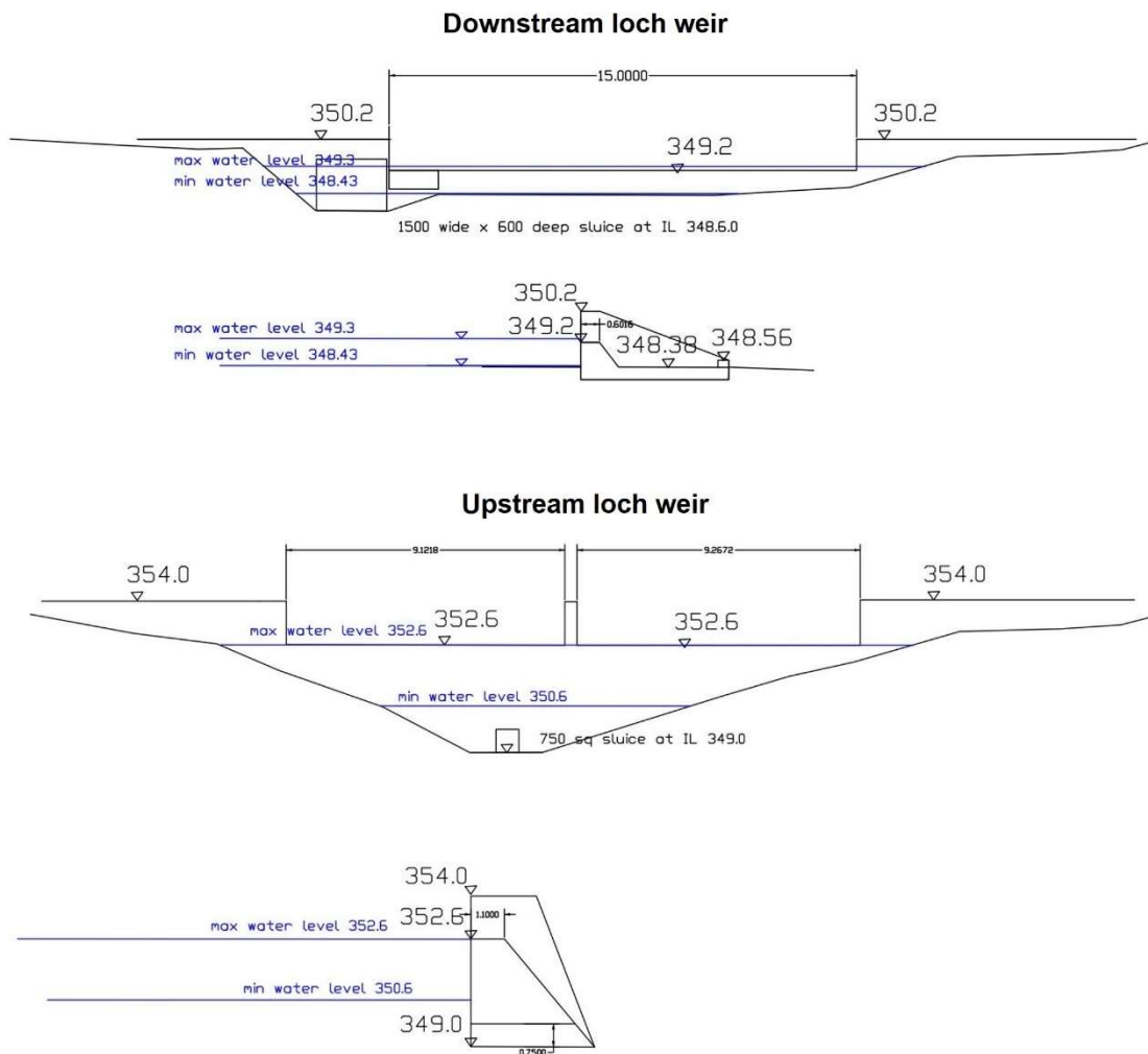
Figure 3.3: Weir configuration drawings for the downstream and upstream Earba Lochs
