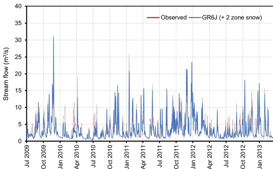
Figure 5.4: Observed and simulated Pattack hydrographs for the calibration period
