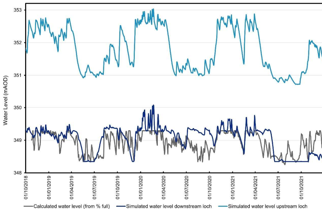
Figure 5.8: Time series of upstream and downstream loch water levels
