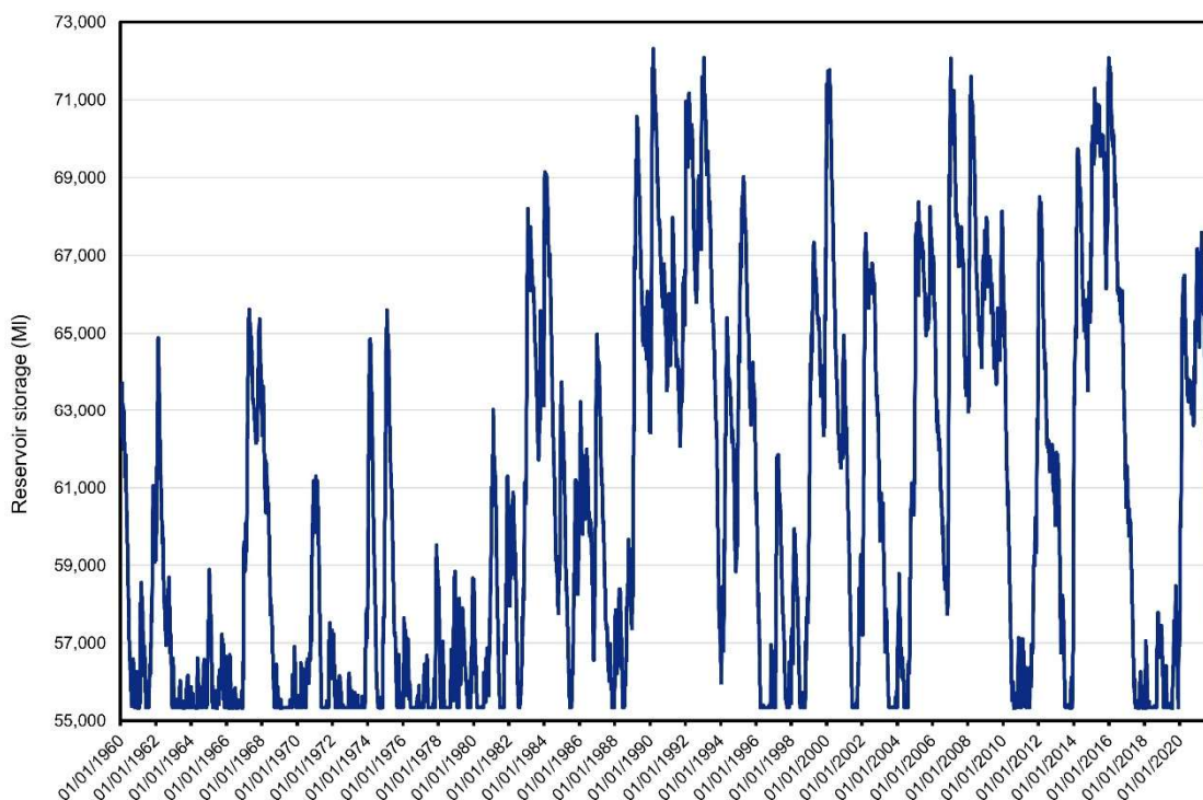
Figure 5.14: Simulated reservoir storage with proposed buffer capacity
