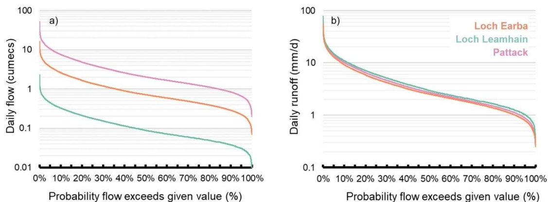
Figure 5.7: Simulated a) flow-duration curves; b) runoff-duration curves for the period 1960-2021
