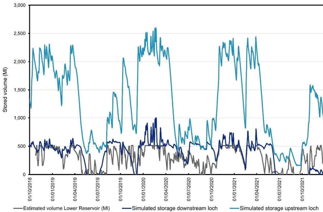
Figure 5.9: Time series of upstream and downstream loch storage volumes
