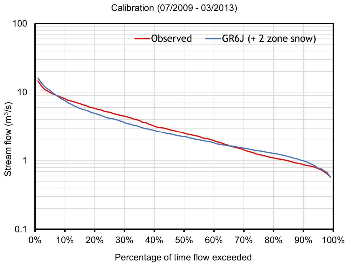
Figure 5.3: Observed and simulated Pattack flow duration curves for the calibration period
