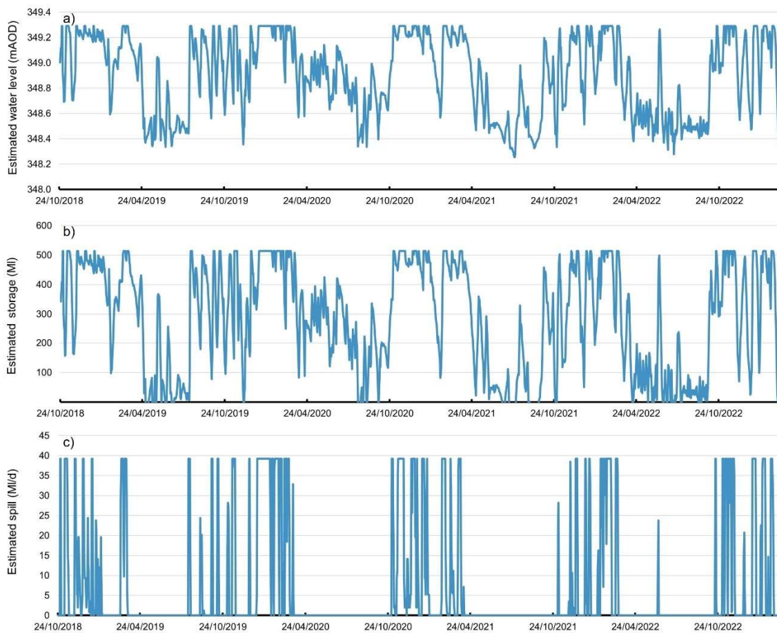
Figure 3.4: Estimated timeseries of a) water level; b) storage; and c) spill at Loch Earba
