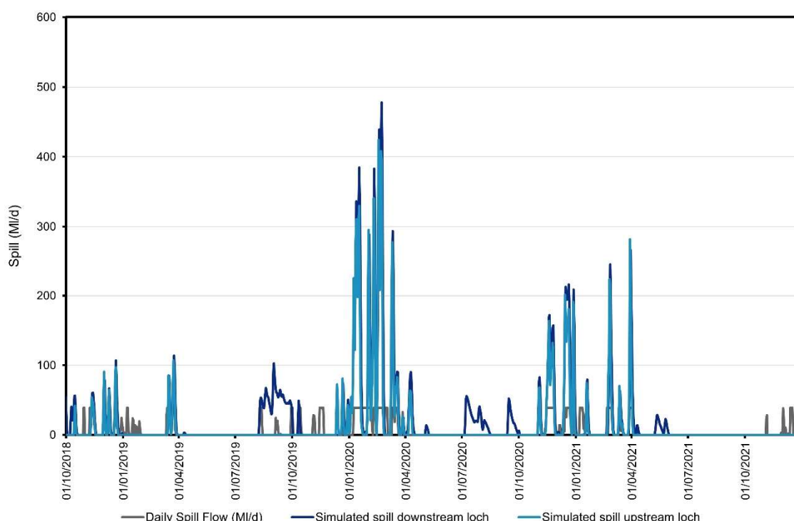
Figure 5.11: Time series of upstream and downstream loch spill estimates
