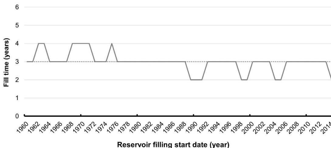
Figure 5.12: Reservoir fill time variability
