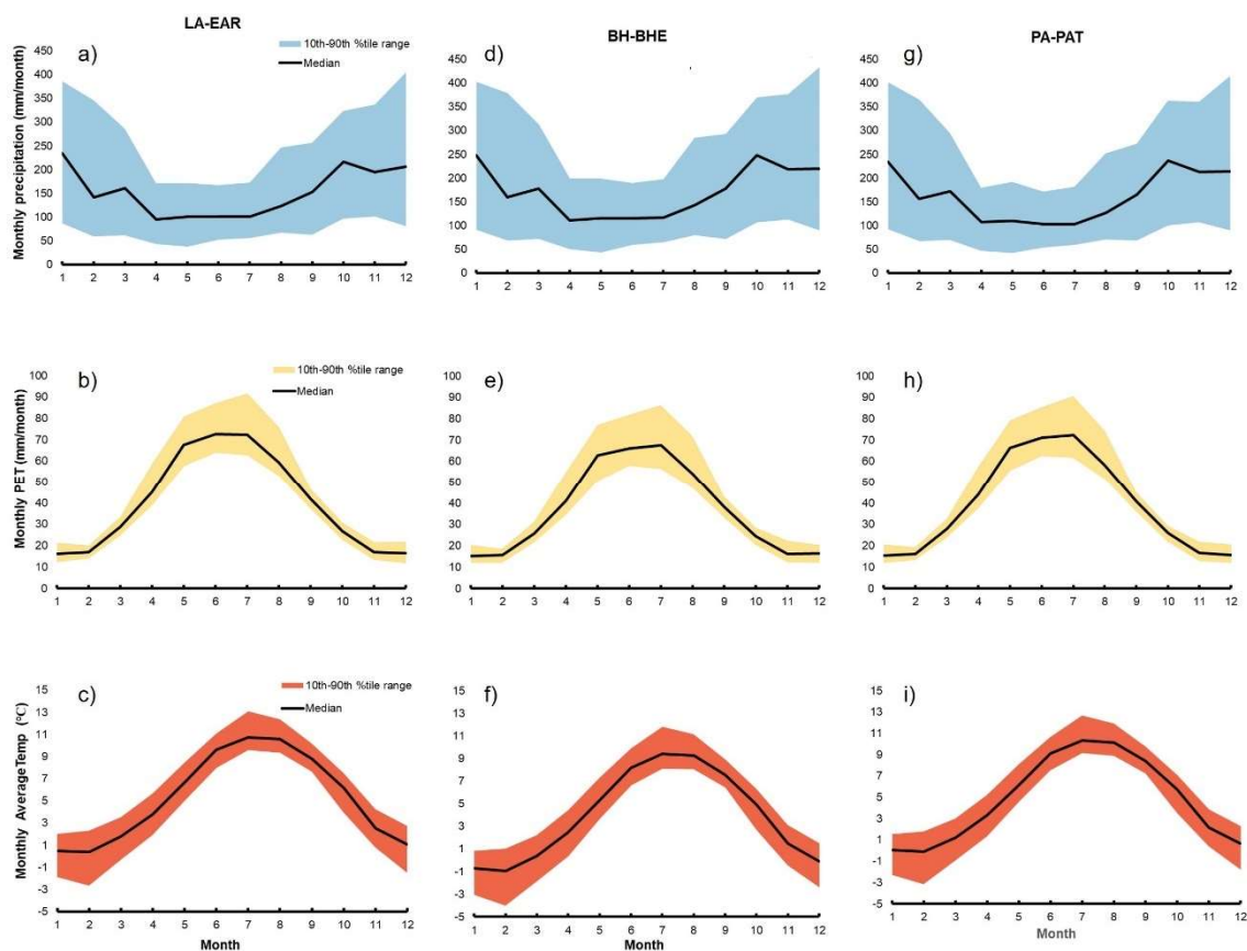
Figure 5.2: Seasonal distribution of a,d,g) total monthly precipitation; b,e,h) total monthly PET; and c,f,i) monthly mean temperatures for the period 1960-2021
