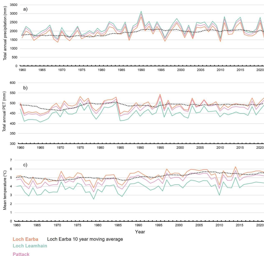
Figure 5.1: Inter-annual variability of a) annual precipitation; b) annual PET; and c) mean temperatures for the period 1960-2021
