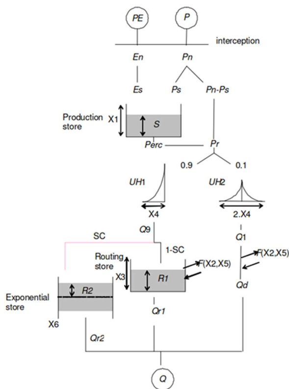
Figure B.1: GR6J model schematic
