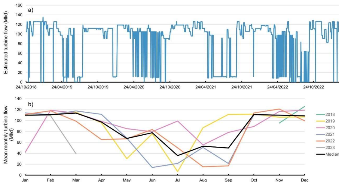
Figure 3.5: a) time series; b) seasonal profiles of estimated turbine flows
