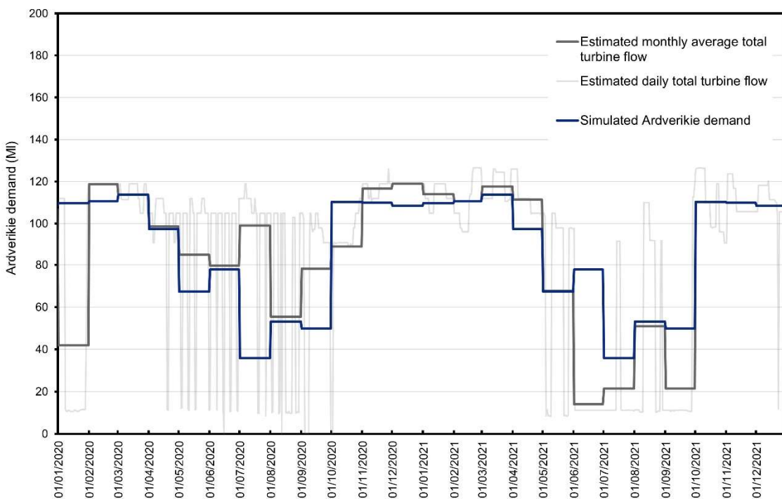
Figure 5.10: Time series of Ardverikie demand
