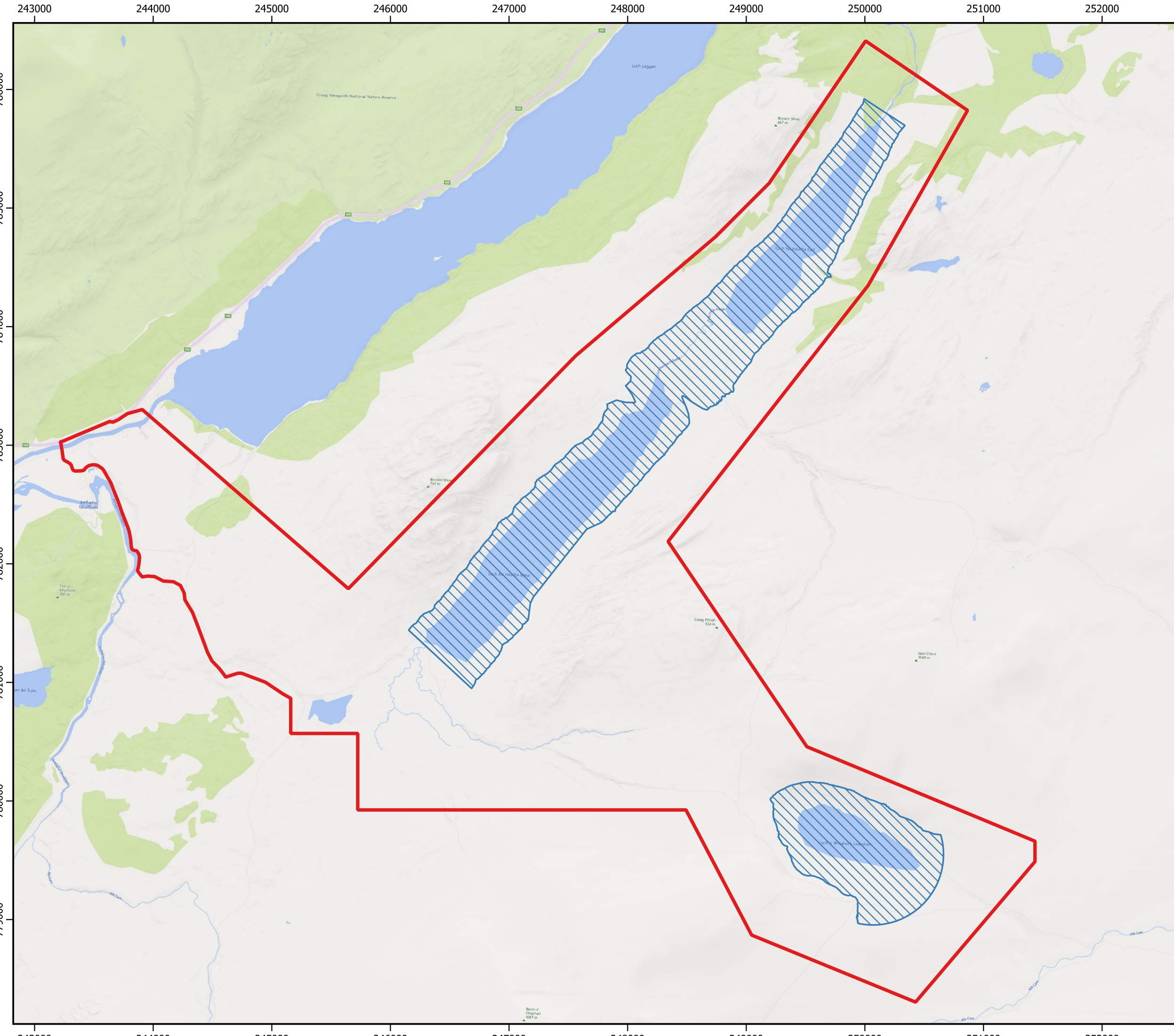
Figure 11.3: Increase in Water Level (Inundation Zone)
