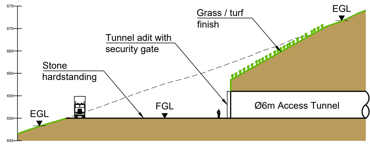
Section A -
