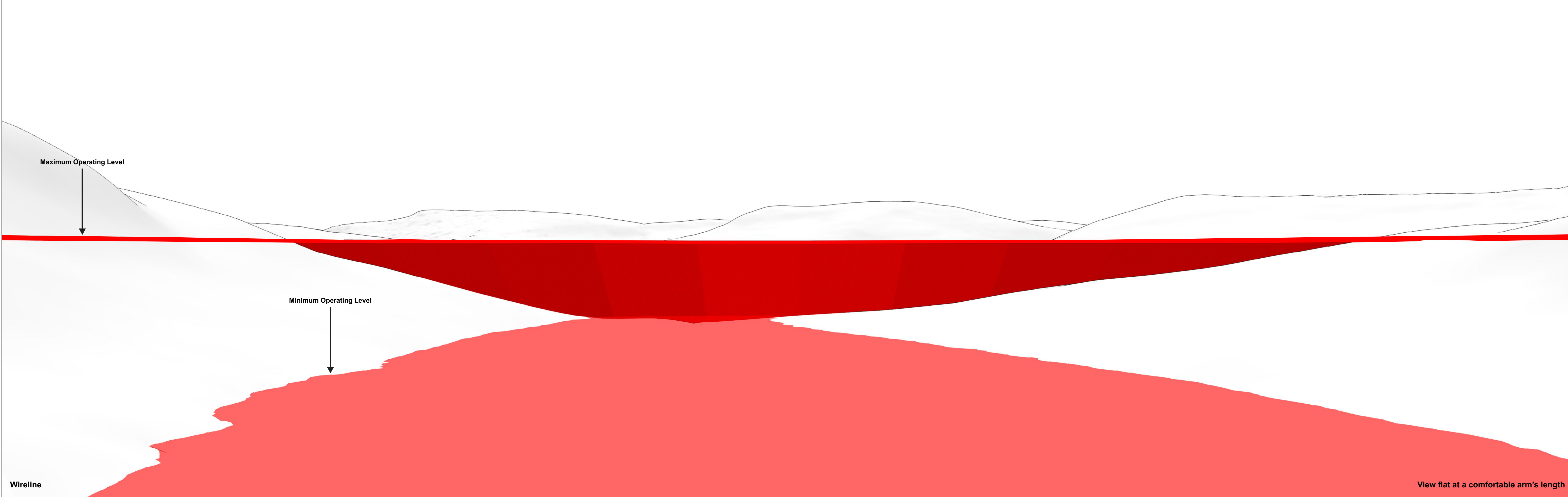
Earba Pumped Storage Hydro Figure 7.5.6b - Representative Wireline: WL2. Loch a' Bhealaich Leamhain - Wireline
